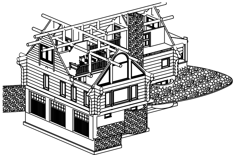
Structural 3-D View
